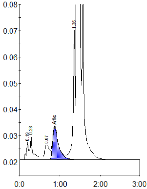
Peak table - ID: 10447827
